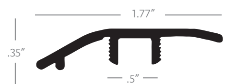
REDUCER
