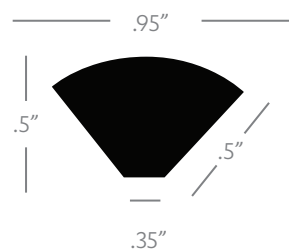
QUARTER ROUND
