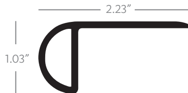
STAIR NOSE
